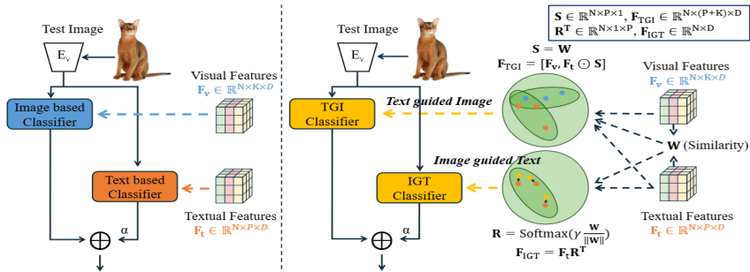
Figure: TIMO Architecture Overview
